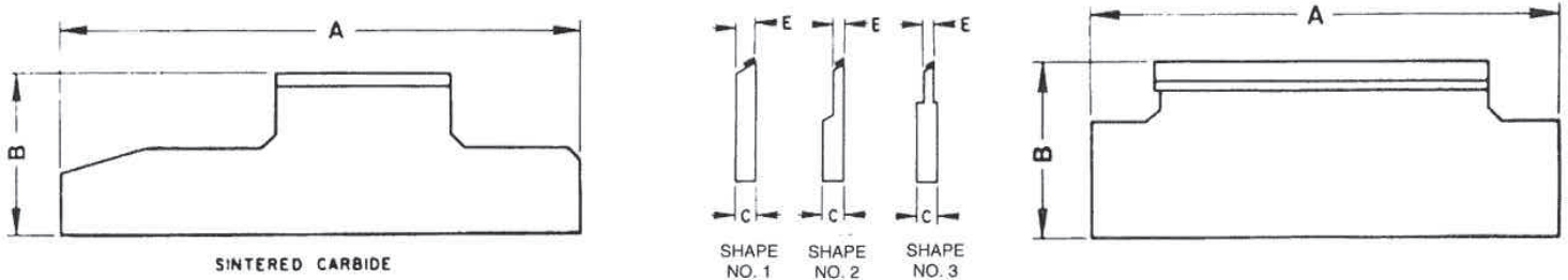
SINTERED CARBIDE
